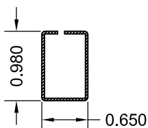
9 SIMRECT1 RAIL/STILE REINFORCEMENT 0.036 GALV. STEEL
