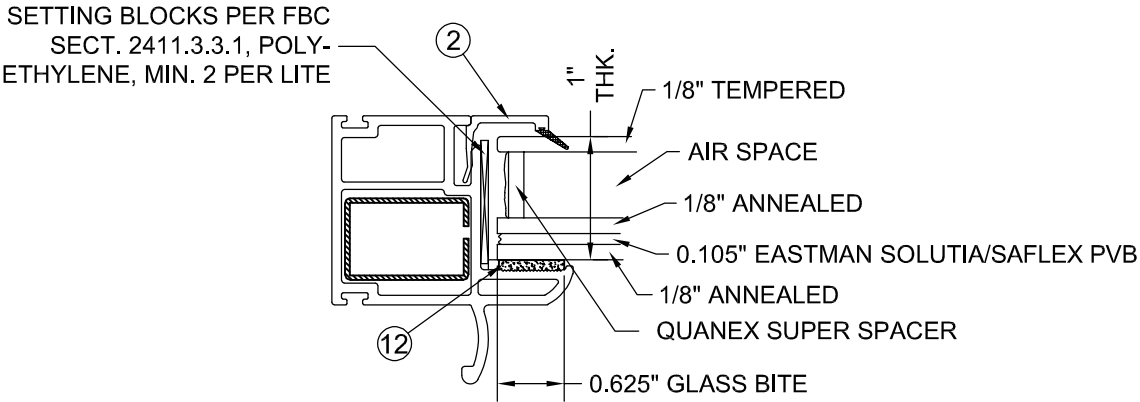
GLAZING DETAIL WITH SOLUTIA/SAFLEX LAMINATE
