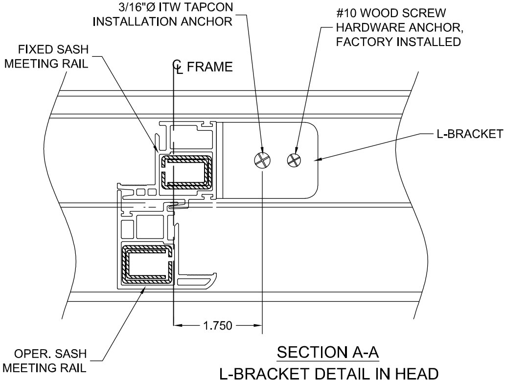
BRACKET AND HARDWARE ANCHOR SUPPLIED BY MANUFACTURER, INSTALLED IN FIELD.
